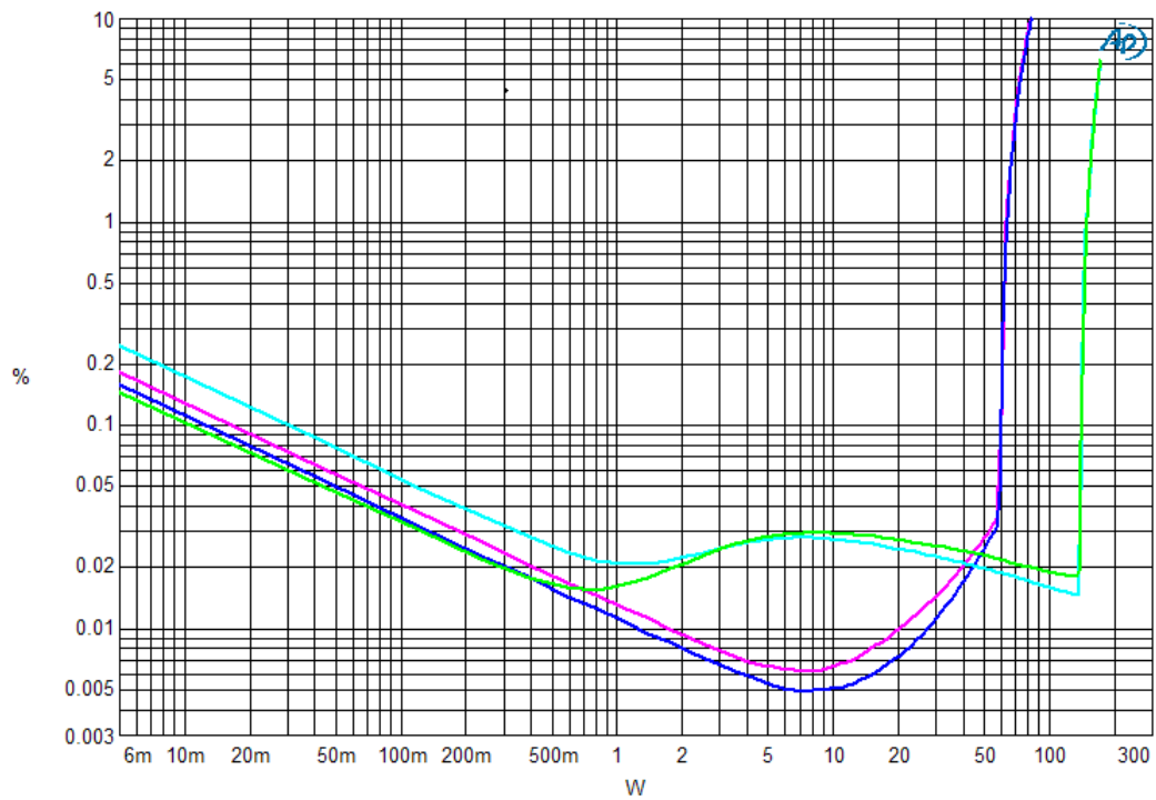
T.H.D + N compared to the output power on 8Ω class A and class AB, 22khz measurement band. (BLUE ch. LEFT class A, PINK ch. RIGHT class A, GREEN ch. LEFT class AB, LIGHT BLUE ch. RIGHT class AB)
