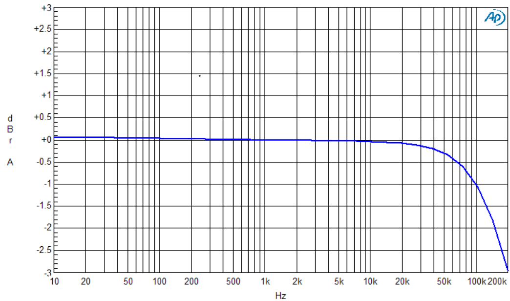
Frequency response at 1W left and right channel
